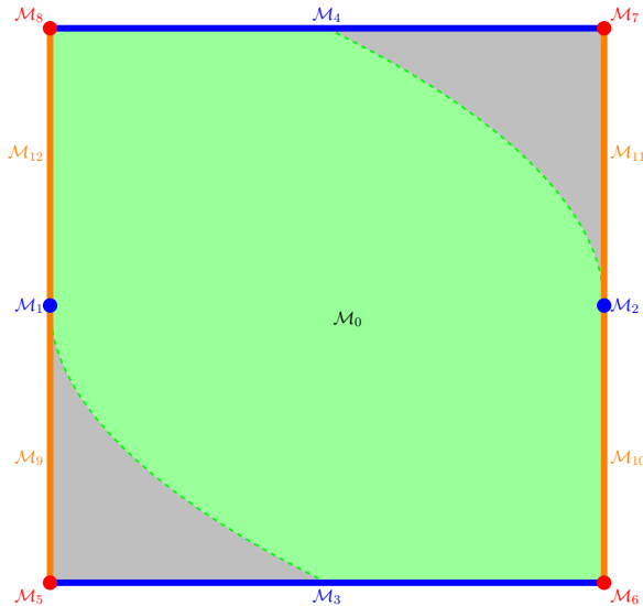
Figure 1: Stratification of Example 2.1.
